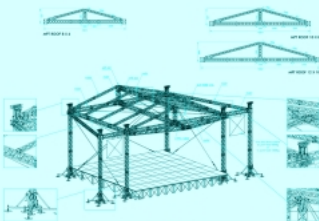
MPT Roof
